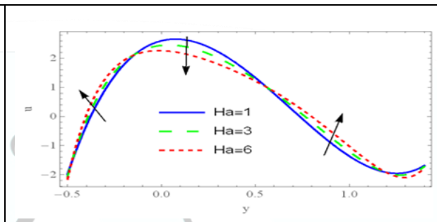
FIGURE2. Behavior of the Hartman number ( H_a ) in a wave frame of the sketch of axial velocity distribution ( n=2, \beta=\pi/6, Da=2, a=0.5, d^*=0.08, b=0.4, \Phi=\pi/6, F0=0.3, F1=1, d=1, W_e=0.6, x=1 )
