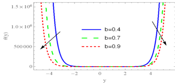
FIGURE16. Behavior of the implitude wave of lower number ( b ) in a wave frame of the sketch of temperature distribution ( n=2 , Ec=1 , Pr=1 , Ha=1 , \beta=\pi/6 , Da=2 , a=0.5 , d^*=0.08 , \Phi=\pi/6 , F0=0.3 , F1=1 , d=1 , W_e=0.6 , x=1 )
