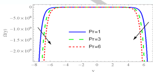
FIGURE22. Behavior of the Prandtl number ( Pr ) in a wave frame of the sketch of consecration distribution ( n=2, Ec=1, Sc=2, Sr=3, Ha=1, \beta=\pi/6, Da=2, a=0.5, d^*=0.08, b=0.4, \Phi=\pi/6, F0=0.3, F1=1, d=1, W_e=0.6, x=1 )
