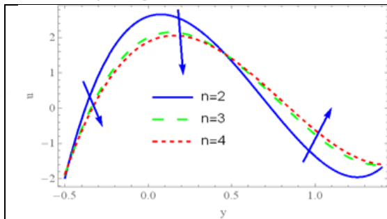
FIGURE1. Behavior of the law number ( n ) in a wave frame of the sketch of axial velocity distribution ( Ha=1, \beta=\pi/6, Da=2, a=0.5, d^*=0.08, b=0.4, \Phi=\pi/6, F0=0.3, F1=1, d=1, W_e=0.6, x=1 )
