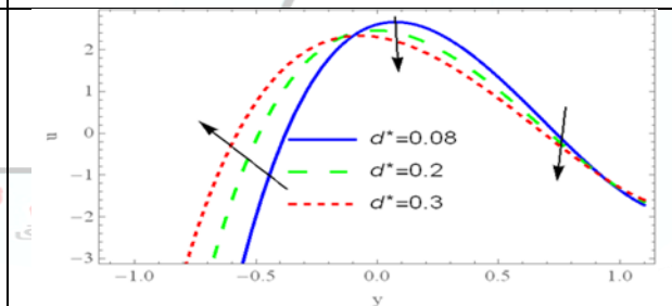
FIGURE4. Behavior of the width number ( d^* ) in a wave frame of the sketch of axial velocity distribution ( n=2, Ha=1, \beta=\pi/6, Da=2, a=0.5, b=0.4, \Phi=\pi/6, F0=0.3, F1=1, d=1, W_e=0.6, x=1 )
