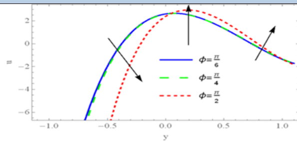
FIGURE6. Behavior of the phase difference ( \phi ) in a wave frame of the sketch of axial velocity distribution ( n=2 , Ha=1 , \beta=\pi/6 , Da=2 , a=0.5 , d^*=0.08 , b=0.4 , F0=0.3 , F1=1 , d=1 , W_e=0.6 , x=1 )
