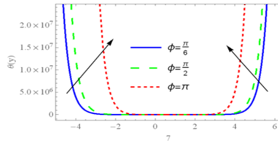
FIGURE17. Behavior of the phase difference ( \phi ) in a wave frame of the sketch of temperature distribution ( n=2 , Ec=1 , Pr=1 , Ha=1 , \beta=\pi/6 , Da=2 , a=0.5 , d^*=0.08 , b=0.4 , F0=0.3 , F1=1 , d=1 , W_e=0.6 , x=1 )
