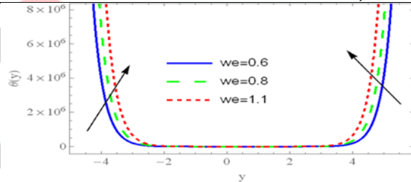
FIGURE19. Behavior of the weissberng number ( W_e ) in a wave frame of the sketch of temperature distribution ( n=2 , Ec=1 , Pr=1 , Ha=1 , \beta=\pi/6 , Da=2 , a=0.5 , d^*=0.08 , b=0.4 , \Phi=\pi/6 , F0=0.3 , F1=1 , d=1 , x=1 )
