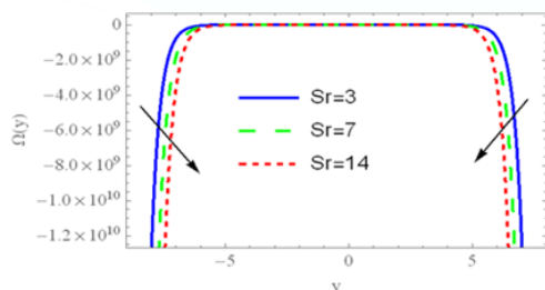
FIGURE24. Behavior of the Soret number ( Sr ) in a wave frame of the sketch of consecration distribution ( n=2, Ec=1, Pr=1, Sc=2, Ha=1, \beta=\pi/6, Da=2, a=0.5, d^*=0.08, b=0.4, \Phi=\pi/6, F0=0.3, F1=1, d=1, W_e=0.6, x=1 )
