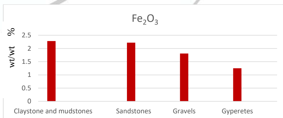
Figure 3: The average of Fe 2 O 3 content of the three localities
