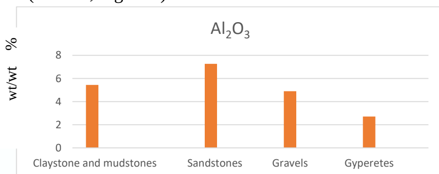
Figure 4: The average of \text{Al}_2\text{O}_3 content of the three localities
