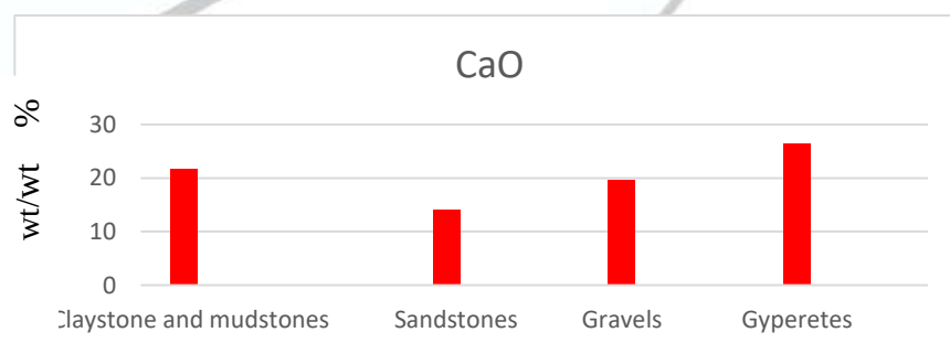
Figure 5: The average of \text{CaO} content of the three localities
